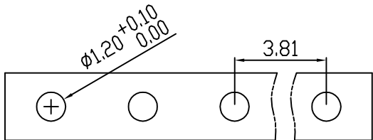
PCB Layout
