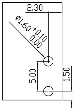
PCB LAYOUT
